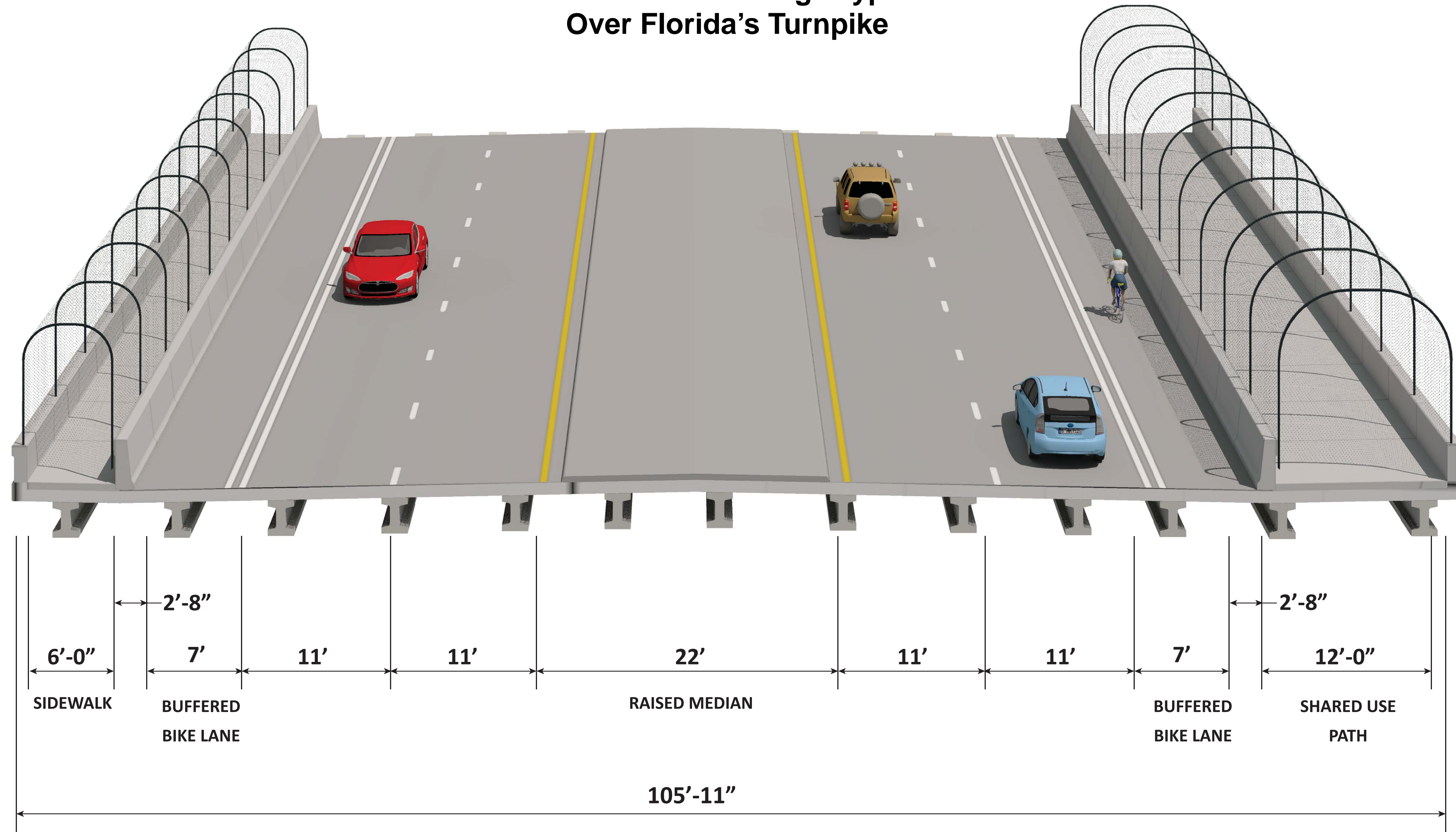
Bridge Improvement
